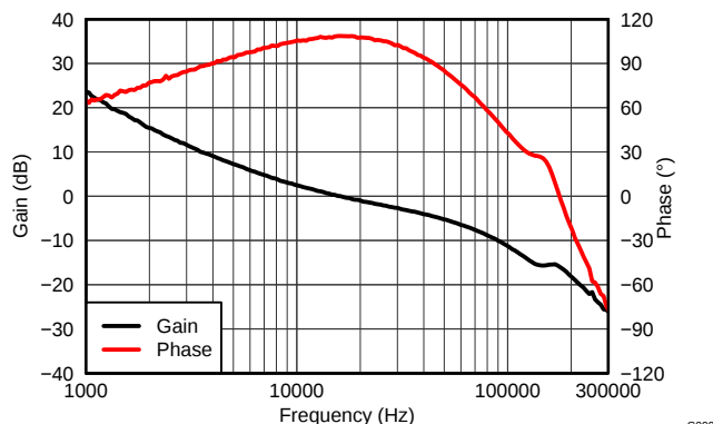
Figure 25. VOUT = 12 V, IOUT = 2 A, COUT1 = 44 \mu F ceramic, COUT2 = 56 \mu F electrolytic, fSW = 800 kHz
