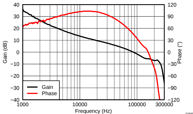
Figure 7. VOUT = 3.3 V, IOUT = 2 A, COUT1 = 44 \mu F ceramic, COUT2 = 56 \mu F electrolytic, fSW = 400 kHz
