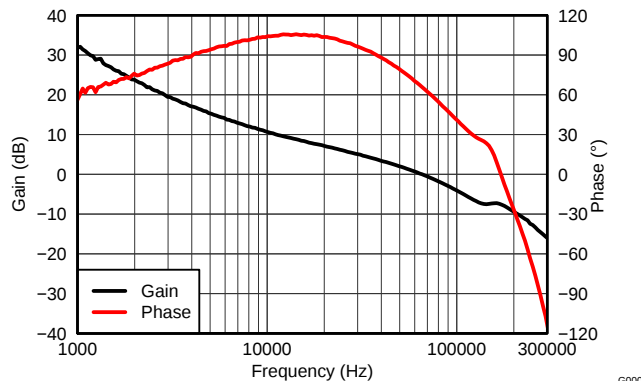
Figure 6. VOUT = 5 V, IOUT = 2 A, COUT1 = 44 \mu F ceramic, COUT2 = 56 \mu F electrolytic, fSW = 500 kHz
