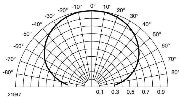
Fig. 11 - Directivity
