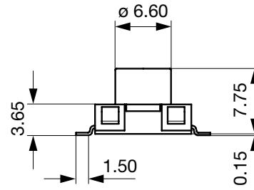
SMS Gullwing Variable height
