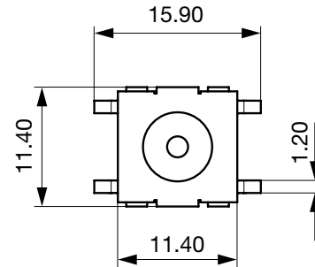
PMS PCB Variable height
