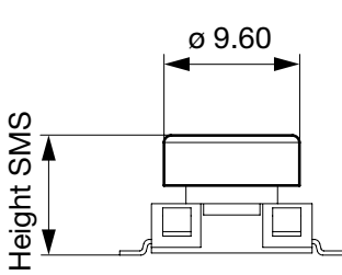
SMS Gullwing with elongated button
