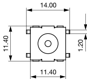
SMS J-lead Variable height
