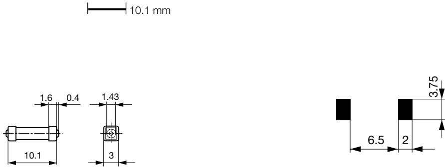
Soldering pads
